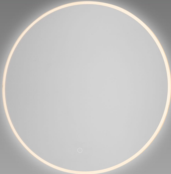
AM324 31.5"D. x 1.25"EXT. 32W LED (Raw 3500lm; Del. 665lm) (Circular Shape)
